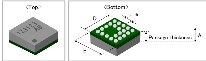
Package outline drawing (example of BGA)
